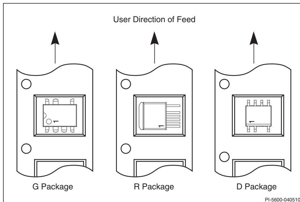
Figure 1. Part Orientation.
