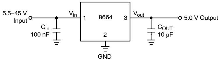
Figure 3. Applications Circuit
