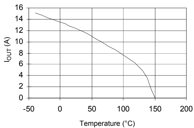
Figure 27. Continuous Current versus Temperature with R_{\theta JA} = 27.5^{\circ}\text{C/W}
